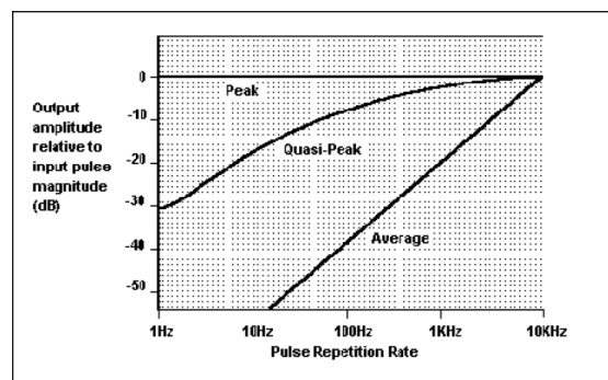
Fig 3. Effect of pulse repetition rate
